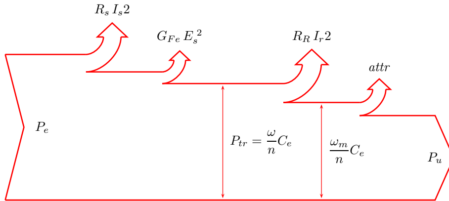
Figure 1: A power scheme for the asynchronous motor
