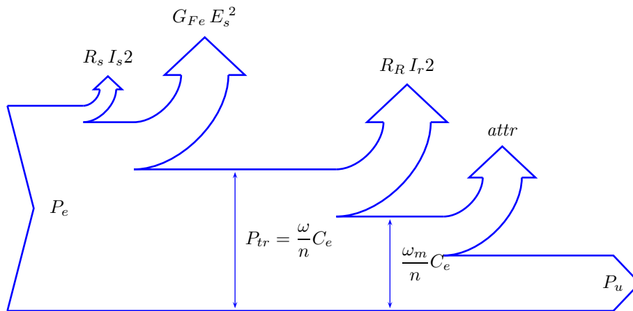
Figure 2: A power scheme for the asynchronous motor
