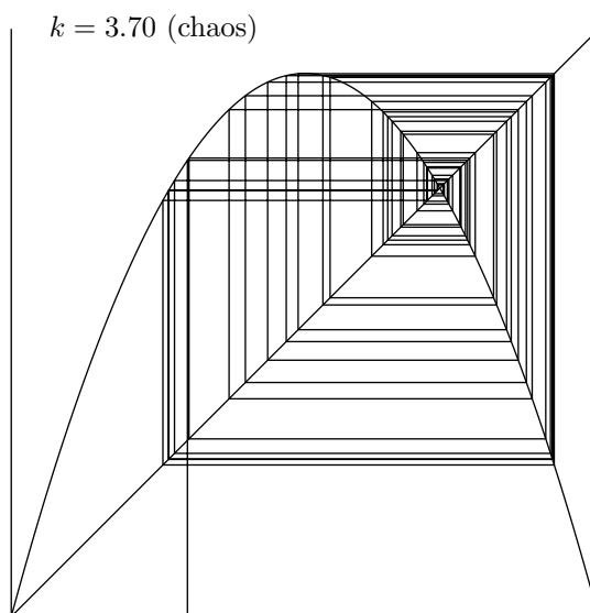
Figure 22: Cobweb plot for the logistic map
