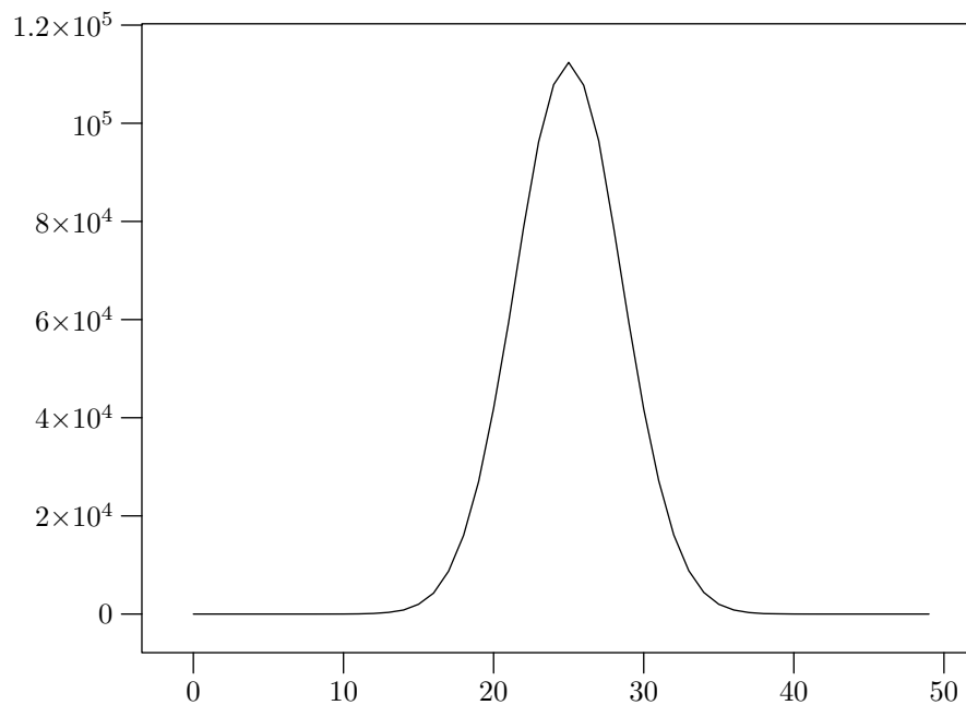
Figure 9: Simulated coin tossing
