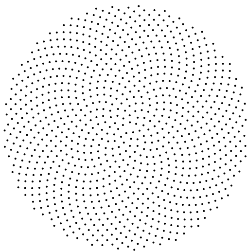
Figure 16: Position of florets in the head of a sunflower
