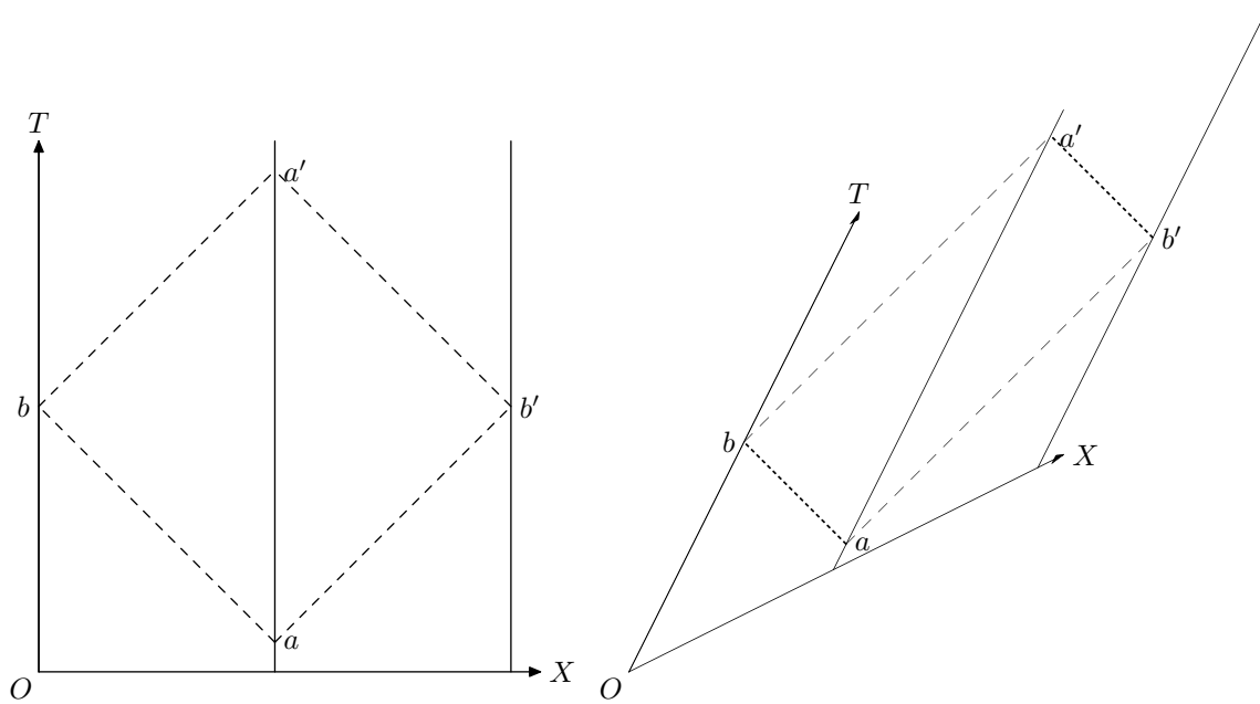
Figure 13: The Lorentz Transformation
