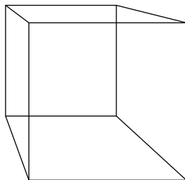
Figure 24: Perspective view of a cube
