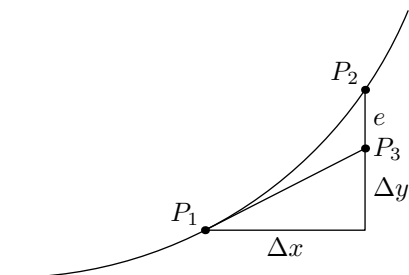
Figure 12: Euler Integration
