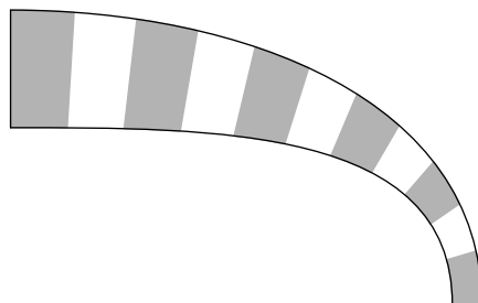
Figure 15: Area reduction in a dissipative system
