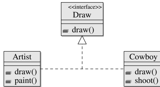
Figure 10: The UML diagram generated from the code in Figure 11
