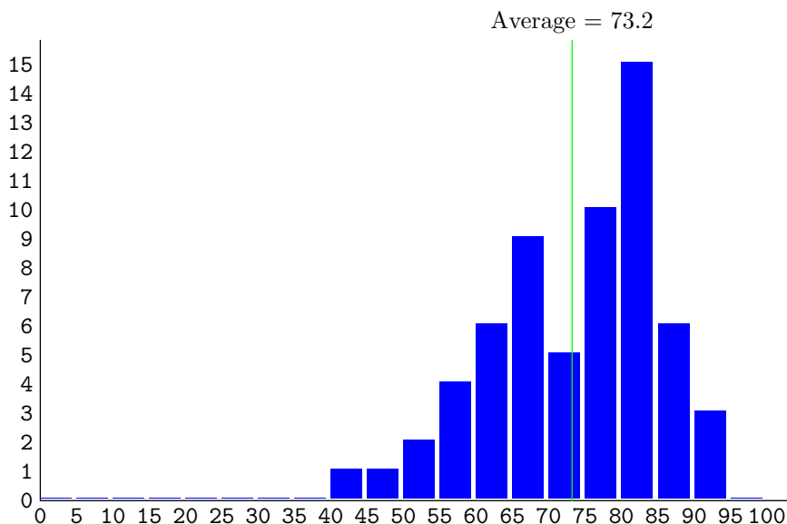
Figure 19: Histogram of Marks
