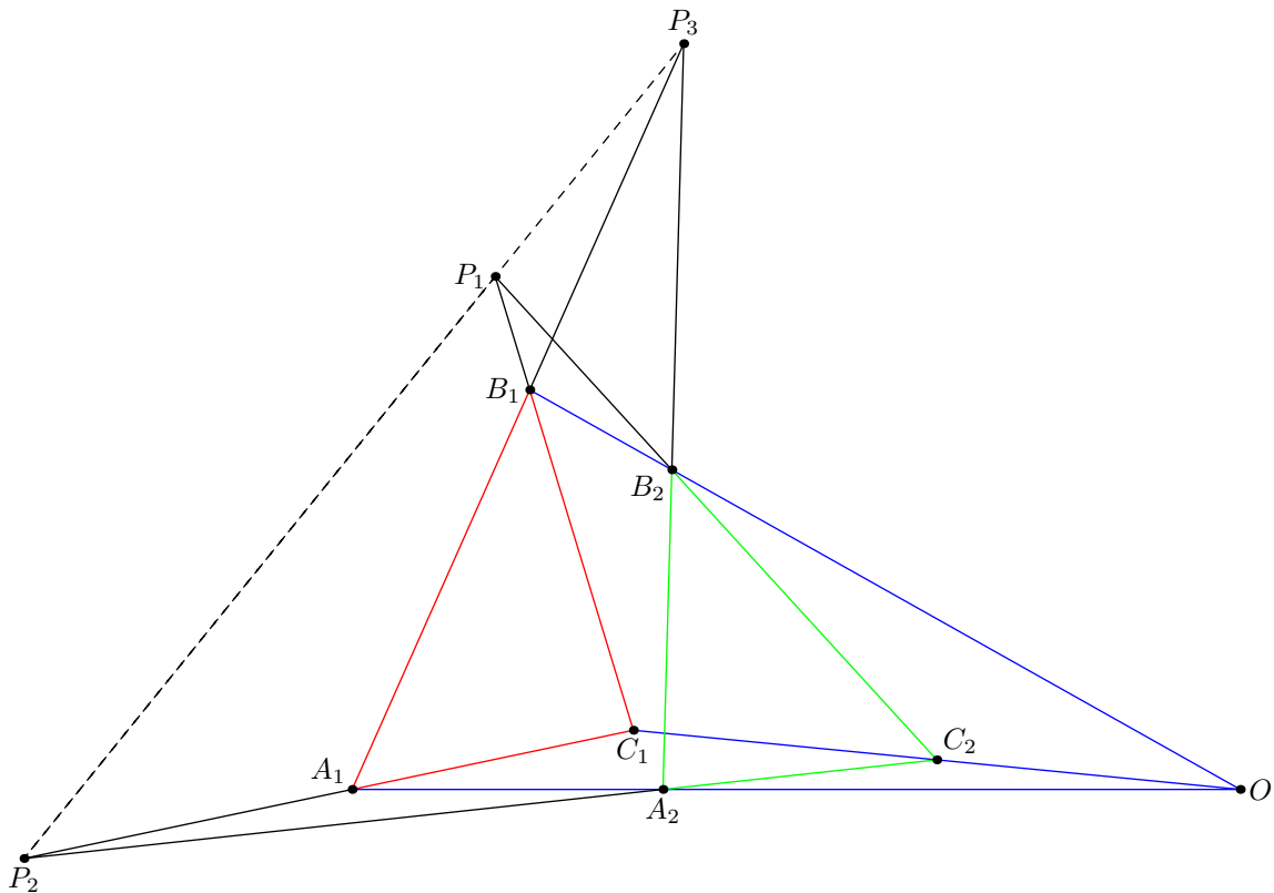
Figure 20: Desargue's Theorem
