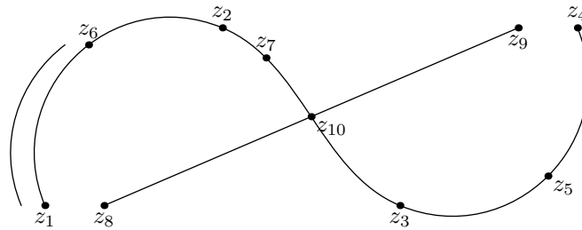
Figure 2: Parametric curves
