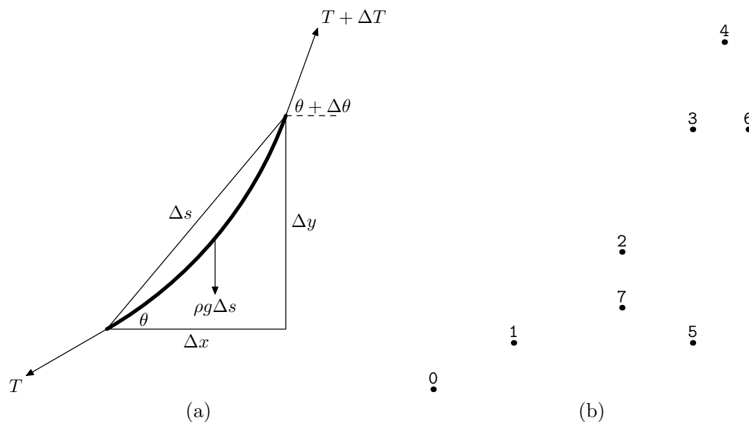
Figure 17: The Hanging Chain: (a) diagram; (b) reference points.
